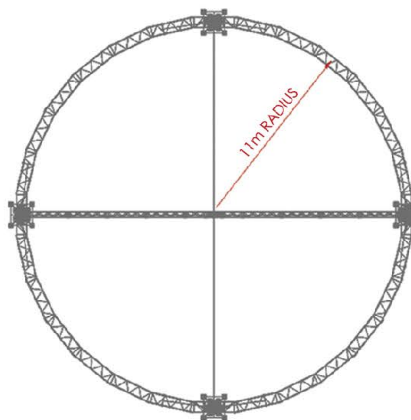
TOP VIEW
