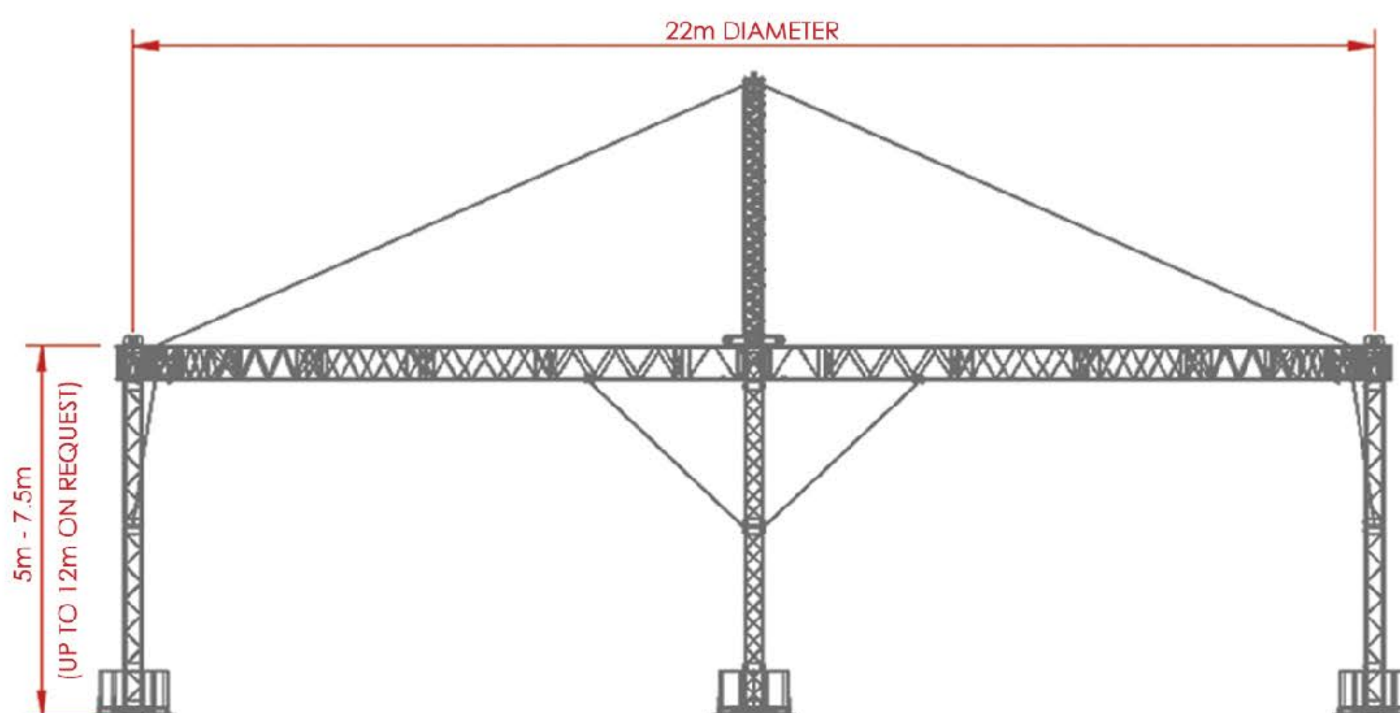
SIDE VIEW
