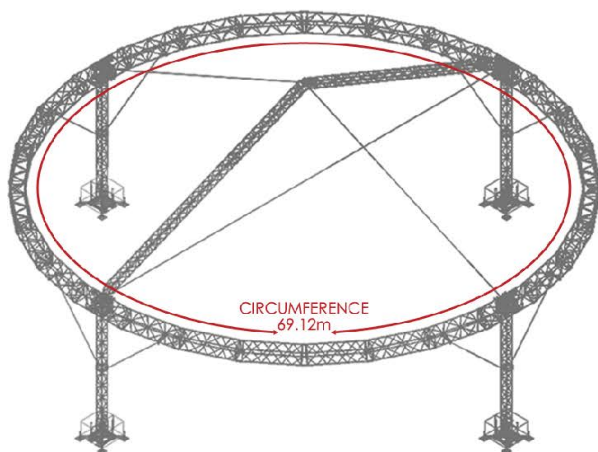
ISOMETRIC VIEW
